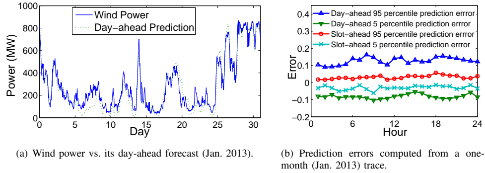
Fig. 10. Wind power and its forecasts.
