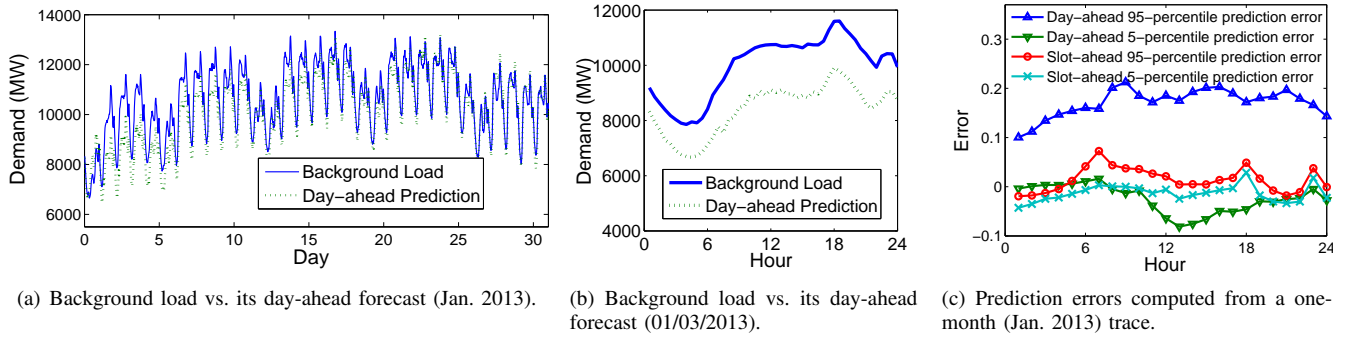
Fig. 9. Background demand and its forecast.
