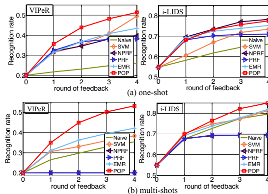
Figure 8. Post-rank optimisation by POP vs. Naïve feedback, and other image retrieval models including NPRF [24], PRF [10], and EMR [23], with \ell_1 -norm as the initial ranking function. The y-axis shows the recognition rate at rank-5 along with the increment of feedback round. (a) one-shot, (b) multi-shots.
