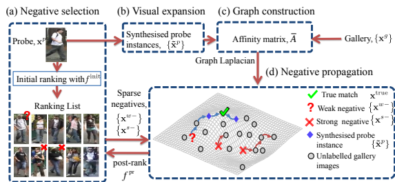
Figure 3. An overview of the proposed one-shot Post-rank OPTimisation (POP) model for person re-identification.
