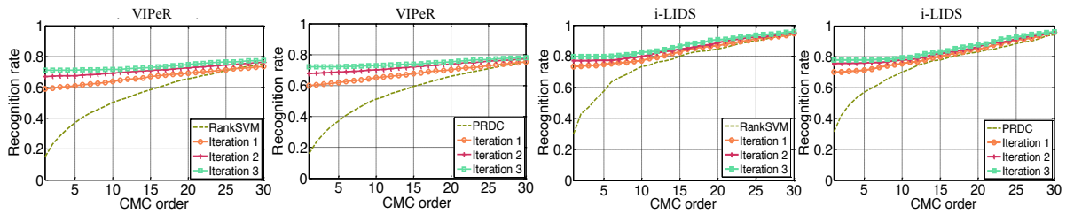
Figure 7. POP post-rank optimisation vs. two re-identification models RankSVM and PRDC (with three rounds of feedback).
