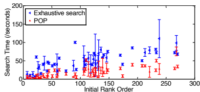
Figure 6. Search time (in second) comparison, between exhaustive search and POP search, both of which are initialised by \ell_1 -norm matching (best viewed in colour).
