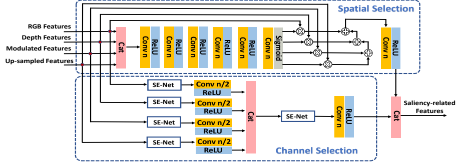
Fig. 4: The detail of AFS module. ‘Cat’ represents the concatenation operation. ‘SE-Net’ is the squeeze-and-excitation network.
