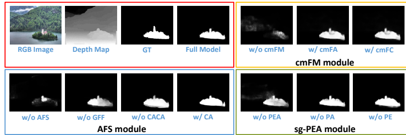
Fig. 9: Visual comparison with different baselines. (1) The baseline w/o cmFM represents our full model without the cmFM module ( i.e. , no modulated features); and the baselines w/ cmFA and w/ cmFC refer to that the cmFM module is replaced by the cmFA or cmFC module ( i.e. , the depth and RGB features are integrated by the element-wise addition or concatenation). (2) The baseline w/o AFS represents our full model without the AFS module ( i.e. , the features after cmFM module are directly concatenated with the up-sampled saliency-related features); the baselines w/o GFF and w/o CACA correspond to removing the fused spatial features and the channel attention-on-channel attention features, respectively; and the baseline w/ CA refers to that the AFS module is replaced by the conventional channel attention module [20]. (3) The baselines w/o PEA , w/o PA , and w/o PE correspond to our full model without the sg-PEA module, the position attention unit, and the edge attention unit, respectively.
