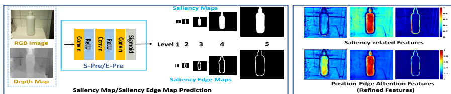
Fig. 6: Visual results of sg-PEA module. Left panel shows the structure of S-Pre/E-Pre unit, and the predicted saliency maps and saliency edge maps in different levels. Right panel shows the intermediate features before and after the sg-PEA module. After the sg-PEA module, the background of features are suppressed, and the edge and position details are assigned more focuses.
